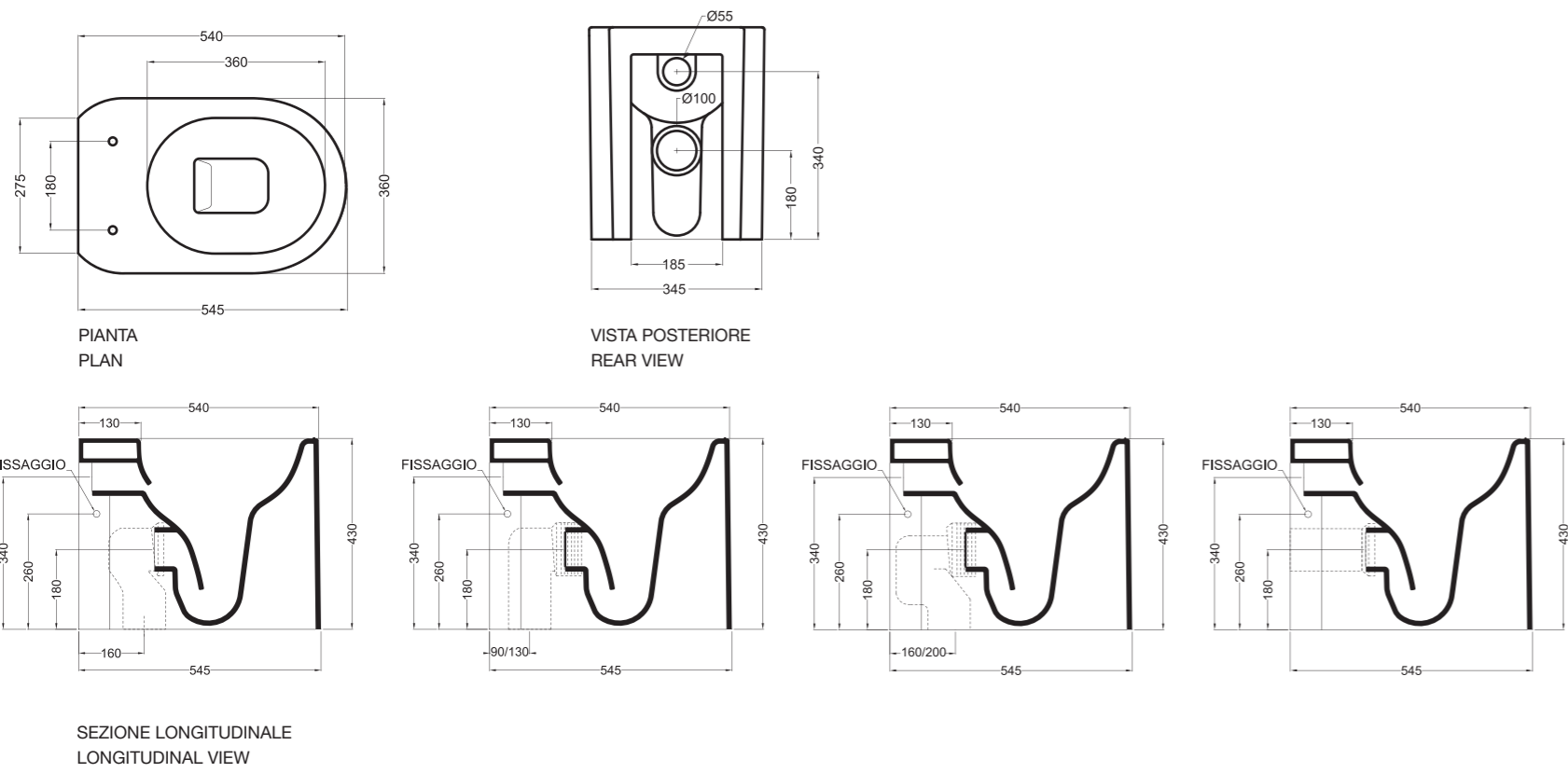
90014 vaso a terra 36x54xH 43 cm_BTW wc 36x54xH 43 cm
