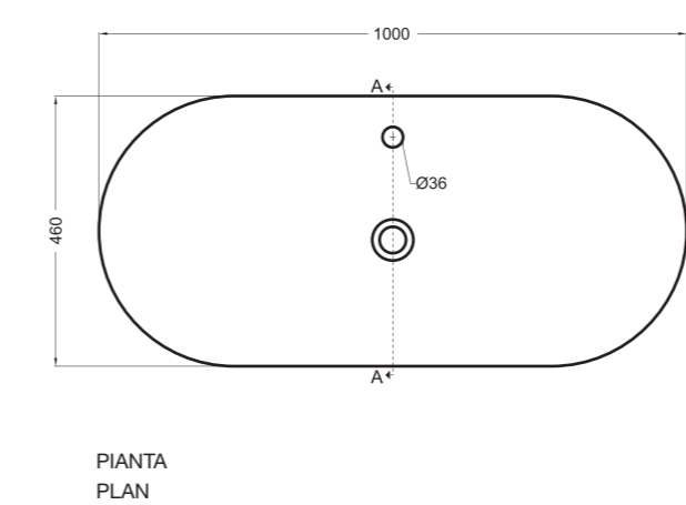
90400 lavabo incasso/sospeso 100x46 cm_inset/wall-hung basin 100x46 cm
