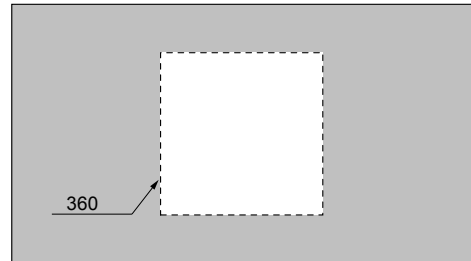
scasso consigliato quadrato 360 x 360 recommended cutting template 360 x 360
